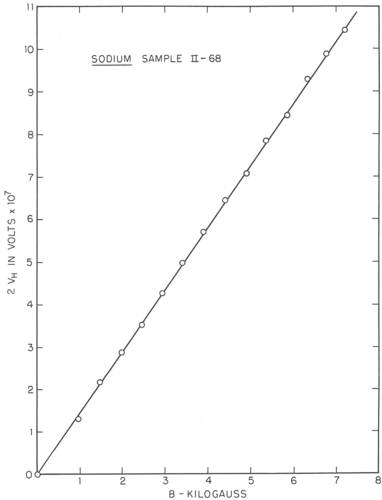
FIG. 3-1 HALL VOLTAGE x 2, 2V_H , VS. MAGNETIC FIELD. A.C. MEASUREMENTS
